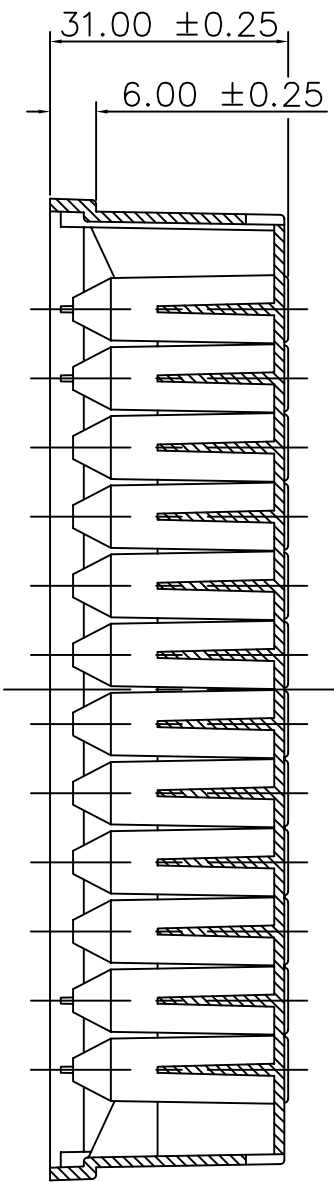
SECTION X-X
