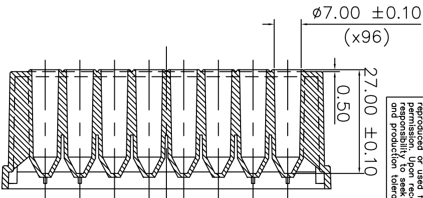
SECTION Y-Y
